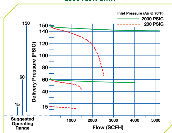
G350 FLOW DATA
